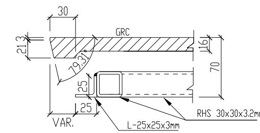
Section-A VAR.=72.5mm
