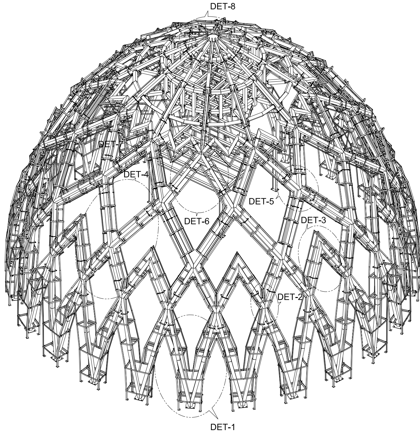
3D VIEW-WITH SUB FRAME
