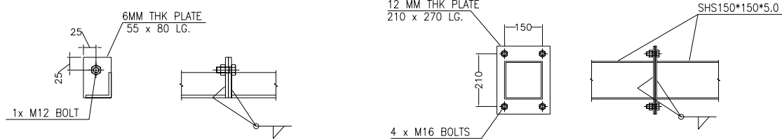
TYPICAL CONNECTION DETAILS
