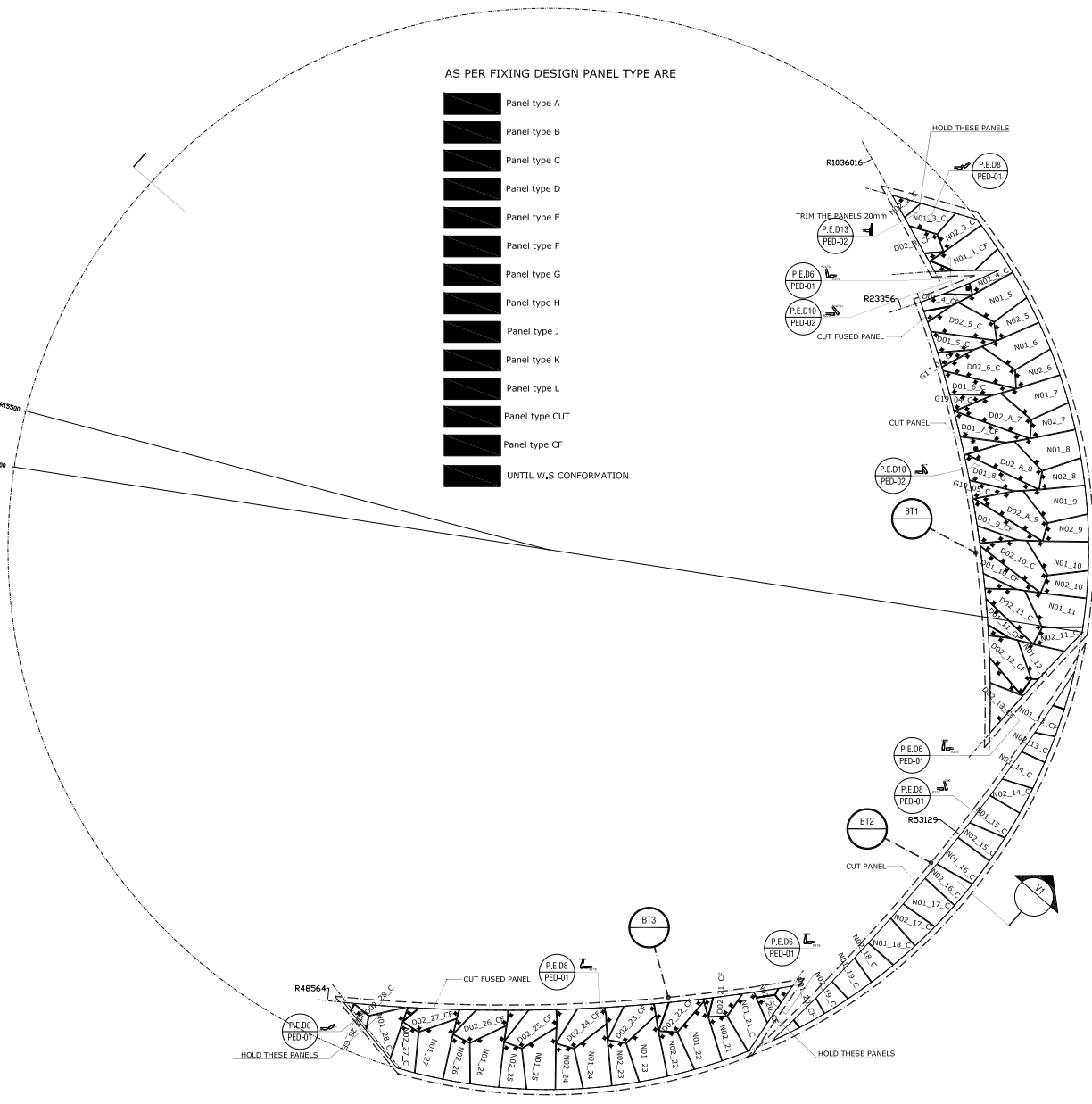
R278 (FBX AR4 ENV CLD ROF R278 SUB) BOTTOM LAYOUT 1/100
