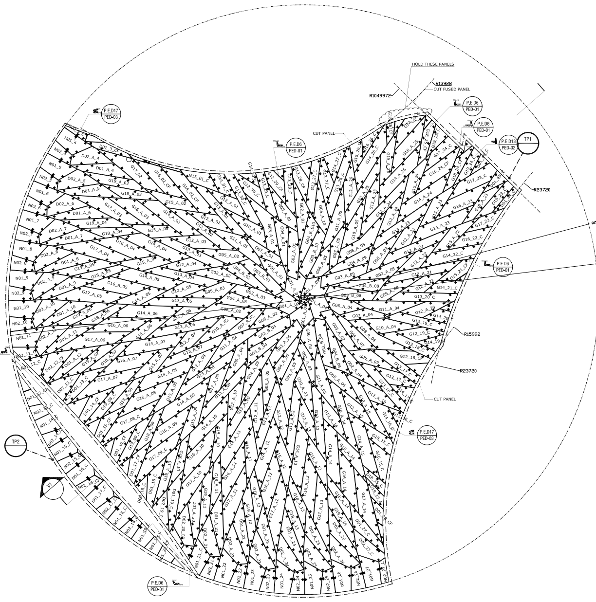
R278 (FBX AR4 ENV CLD ROF R278 SUB) TOP LAYOUT 1/100
